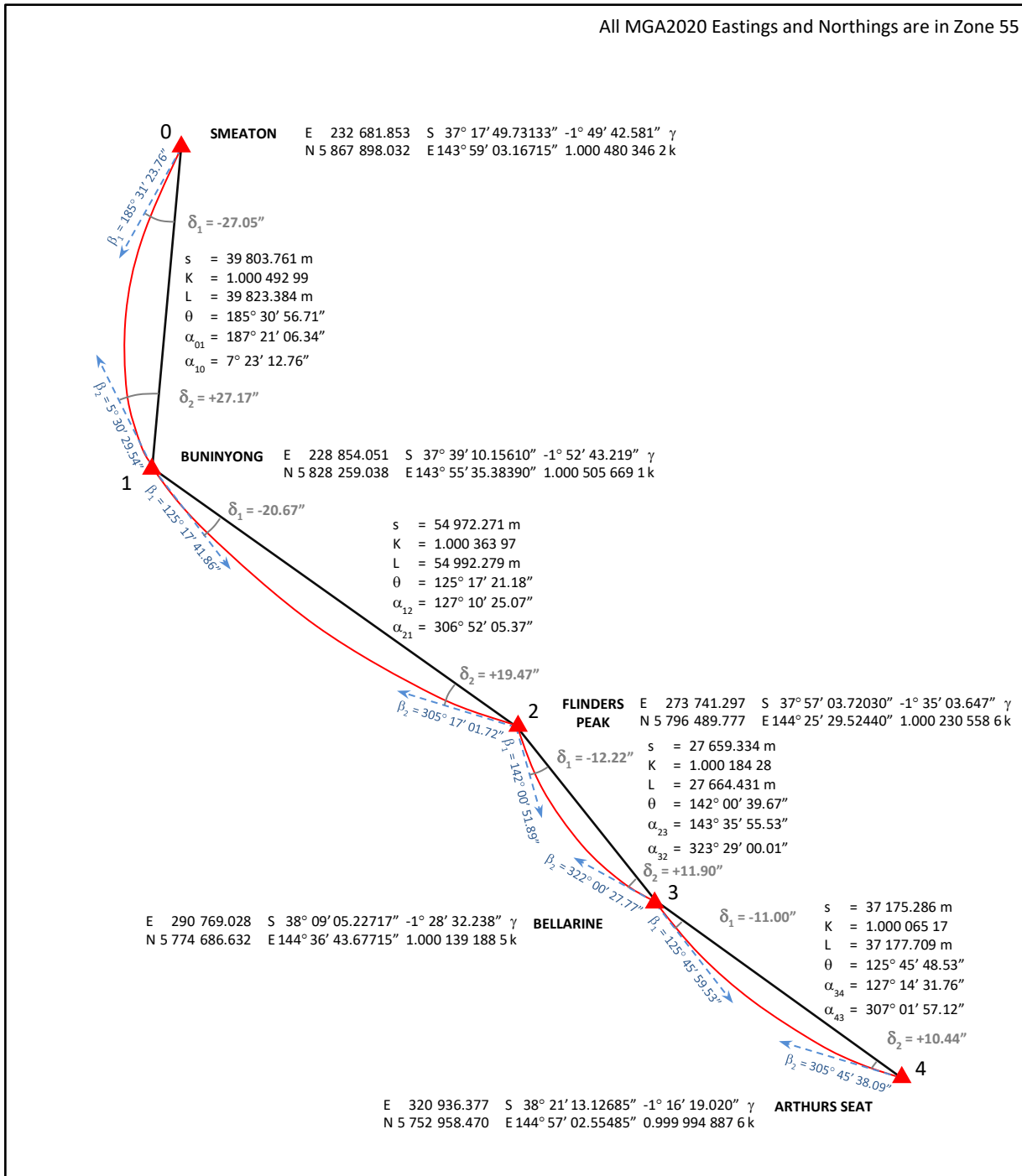
Figure C.2 Traverse diagram.
